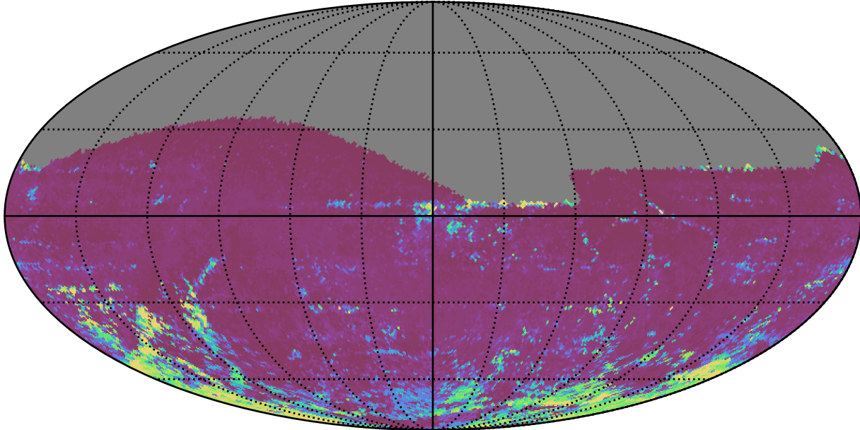
ddf_loaded_half_fl1_v3.4_10yrs All sky i band: 75th Percentile Intranight Timespan
