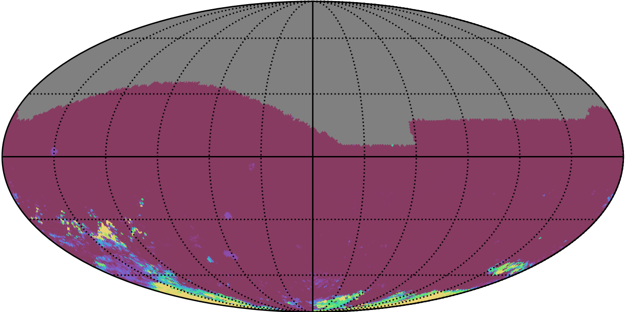
ddf_loaded_half_fl1_v3.4_10yrs All sky gr bands: 75th Percentile Intranight Timespan
