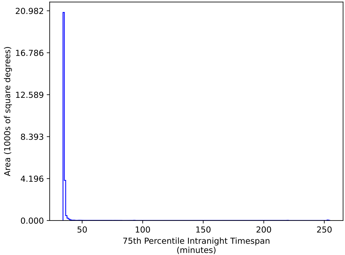
ddf_loaded_half_fl1_v3.4_10yrs All sky gr bands: 75th Percentile Intranight Timespan
