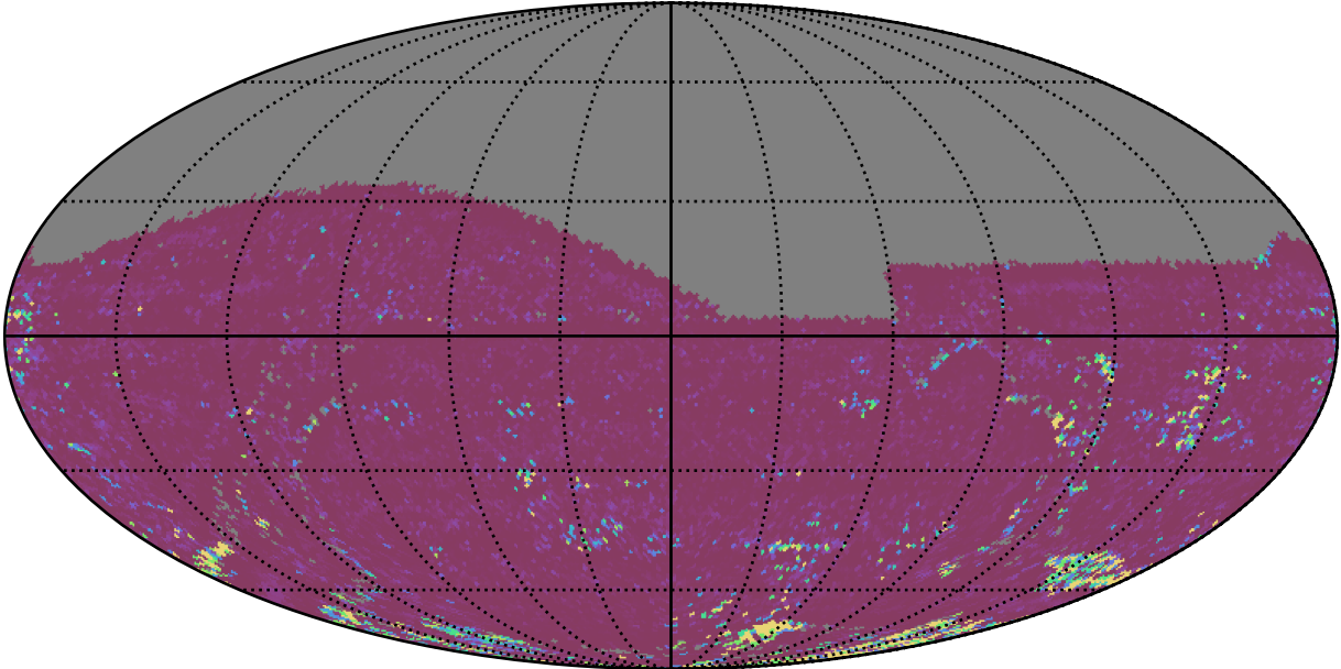
ddf_loaded_half_fl1_v3.4_10yrs All sky g band: 75th Percentile Intranight Timespan
