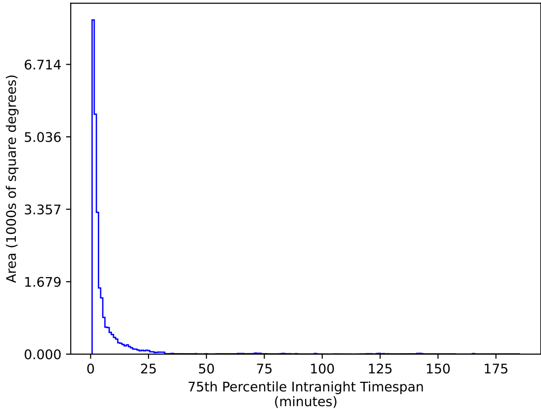
ddf_loaded_half_fl1_v3.4_10yrs All sky g band: 75th Percentile Intranight Timespan
