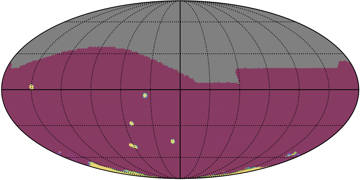
ddf_loaded_half_fl1_v3.4_10yrs All sky all bands: 75th Percentile Intranight Timespan
