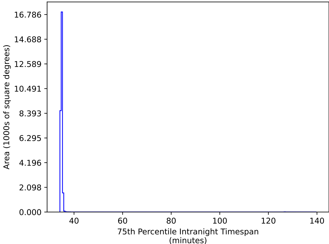
ddf_loaded_half_fl1_v3.4_10yrs All sky all bands: 75th Percentile Intranight Timespan
