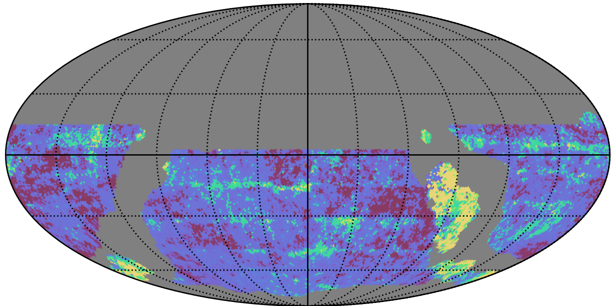
ddf_loaded_half_fl1_v3.4_10yrs WFD y band: 20thPercentile Inter-Night Gap
