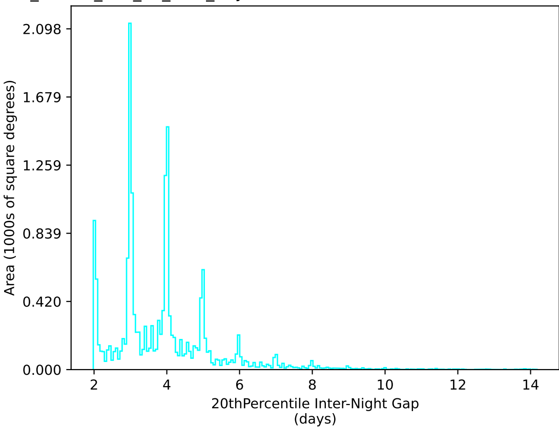
ddf_loaded_half_fl1_v3.4_10yrs WFD u band: 20thPercentile Inter-Night Gap
