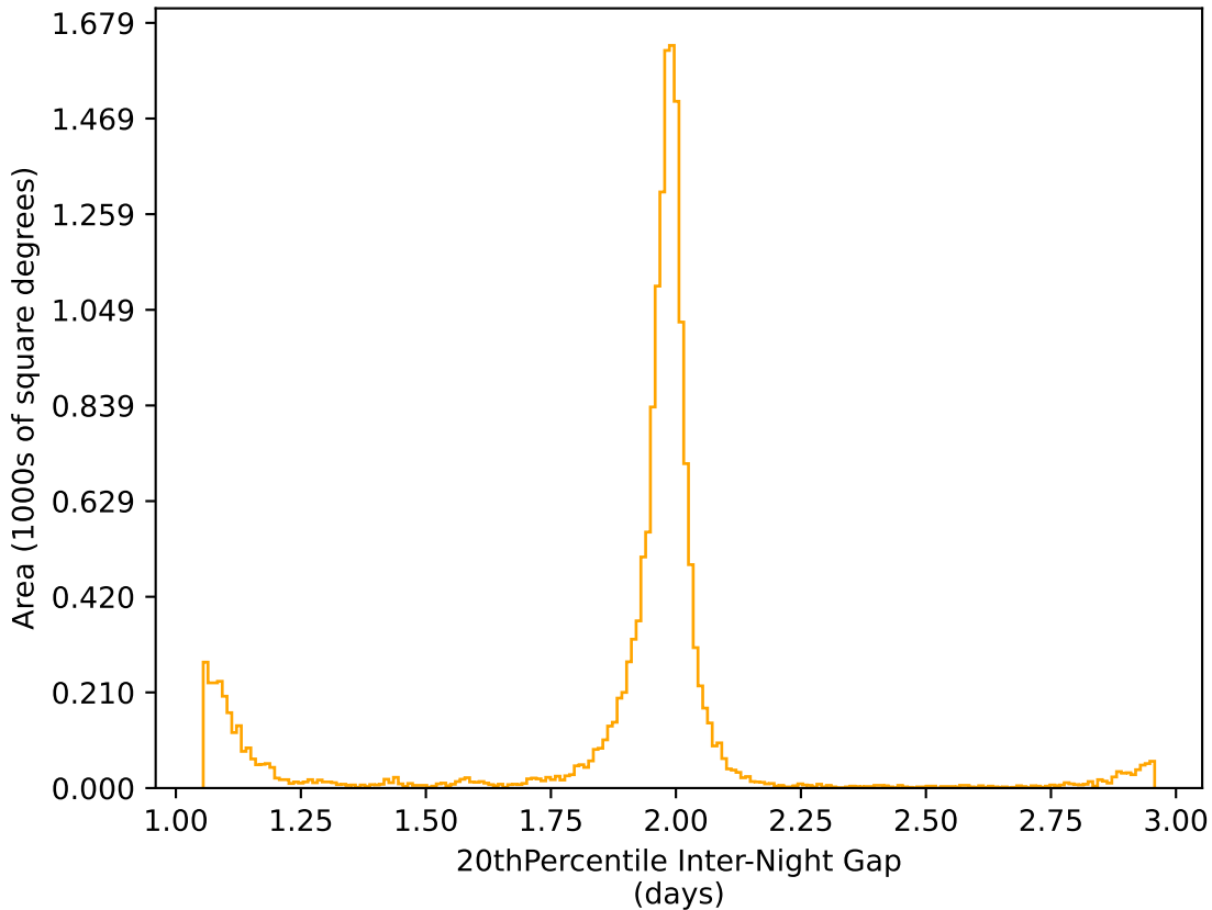
ddf_loaded_half_fl1_v3.4_10yrs WFD r band: 20thPercentile Inter-Night Gap
