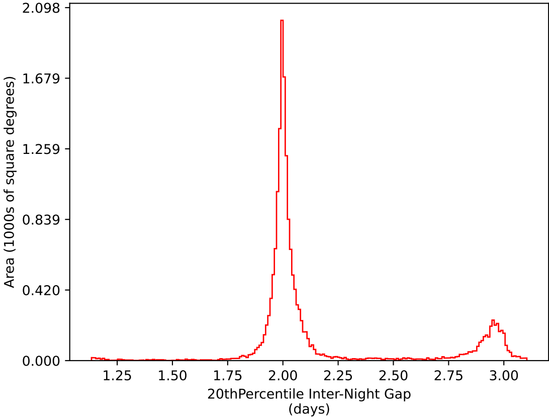
ddf_loaded_half_fl1_v3.4_10yrs WFD i band: 20thPercentile Inter-Night Gap
