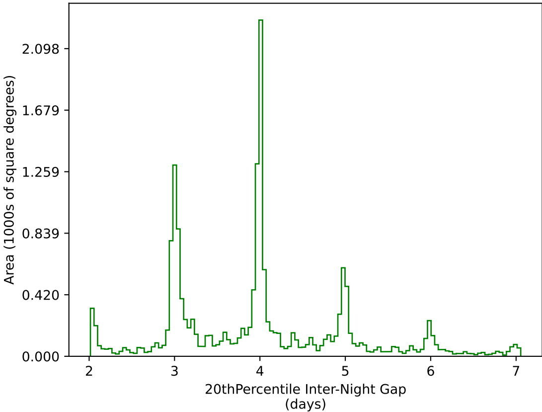
ddf_loaded_half_fl1_v3.4_10yrs WFD g band: 20thPercentile Inter-Night Gap
