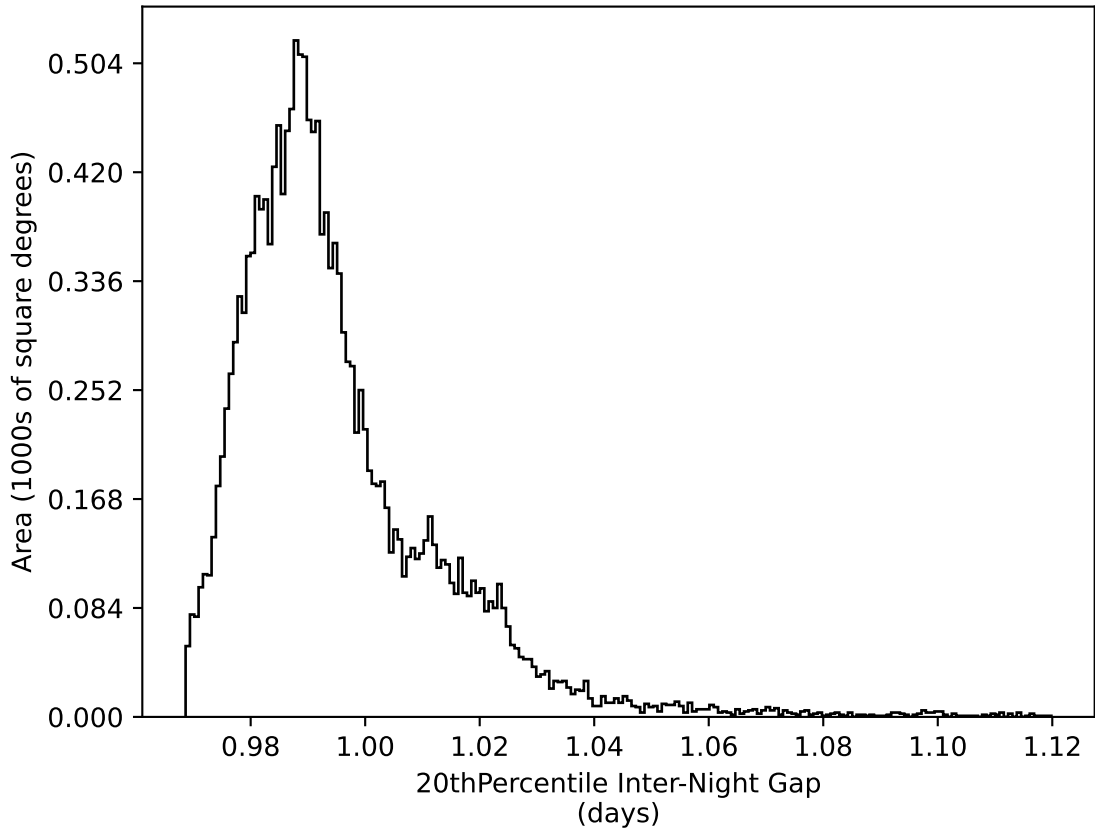
ddf_loaded_half_fl1_v3.4_10yrs WFD all bands: 20thPercentile Inter-Night Gap
