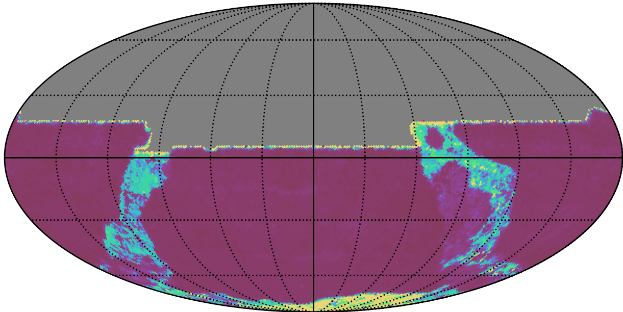
ddf_loaded_half_fl1_v3.4_10yrs All sky y band: 20thPercentile Inter-Night Gap
