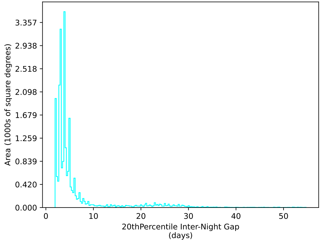
ddf_loaded_half_fl1_v3.4_10yrs All sky u band: 20thPercentile Inter-Night Gap
