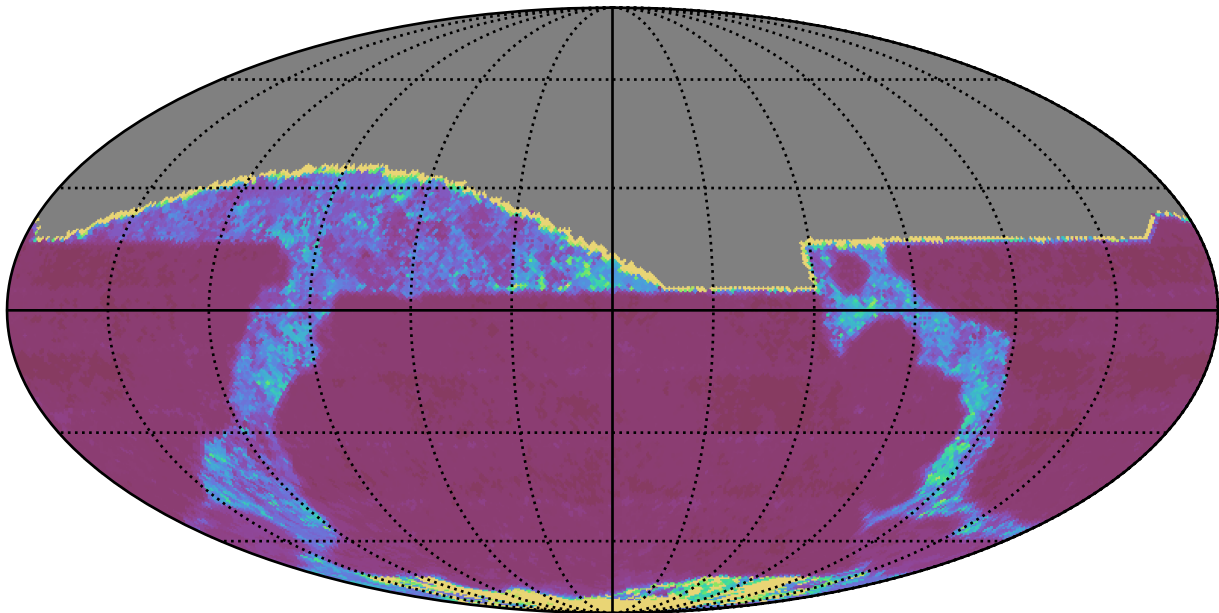
ddf_loaded_half_fl1_v3.4_10yrs All sky r band: 20thPercentile Inter-Night Gap
