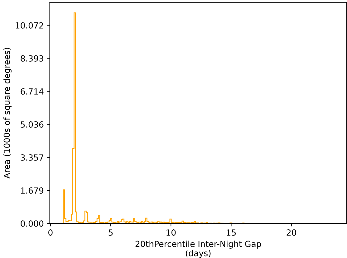
ddf_loaded_half_fl1_v3.4_10yrs All sky r band: 20thPercentile Inter-Night Gap
