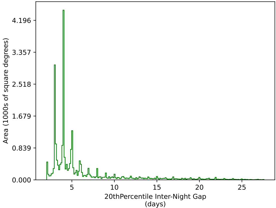
ddf_loaded_half_fl1_v3.4_10yrs All sky g band: 20thPercentile Inter-Night Gap
