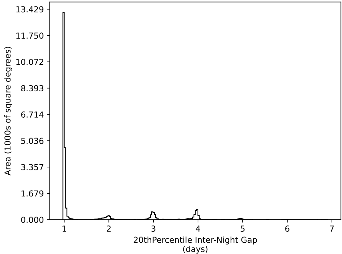
ddf_loaded_half_fl1_v3.4_10yrs All sky all bands: 20thPercentile Inter-Night Gap
