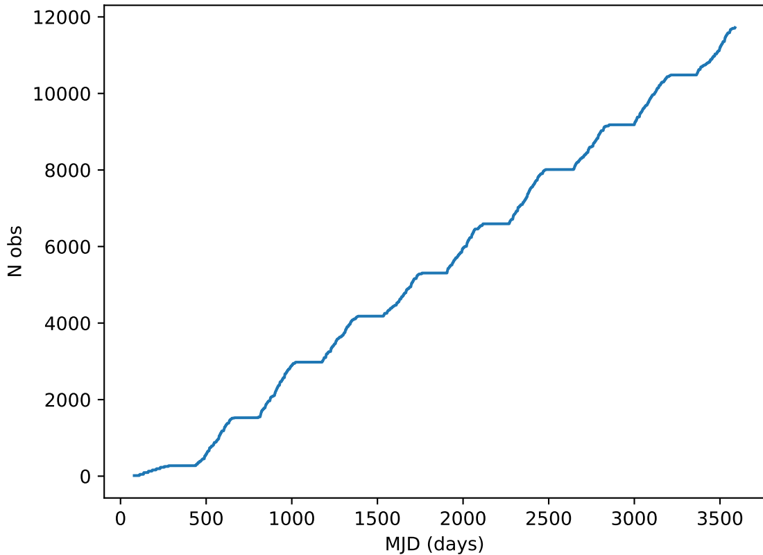
ddf_loaded_half_fl1_v3.4_10yrs all bands: DD:XMM_LSS Cumulative NVisits
