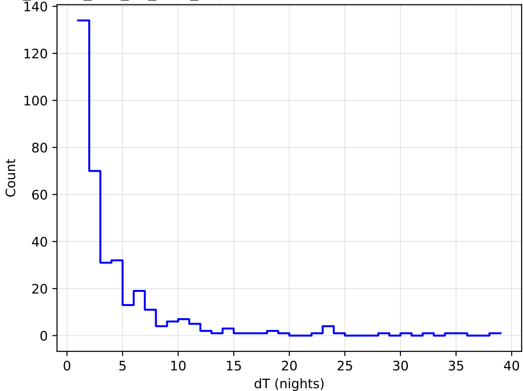
ddf_loaded_half_fl1_v3.4_10yrs all bands: DD:WFD Delta Nights Histogram
