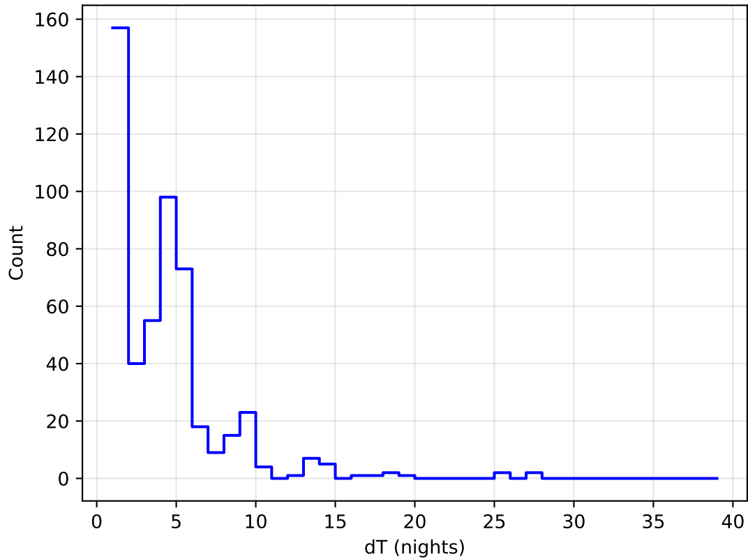
ddf_loaded_half_fl1_v3.4_10yrs all bands: DD:ELAISS1 Delta Nights Histogram
