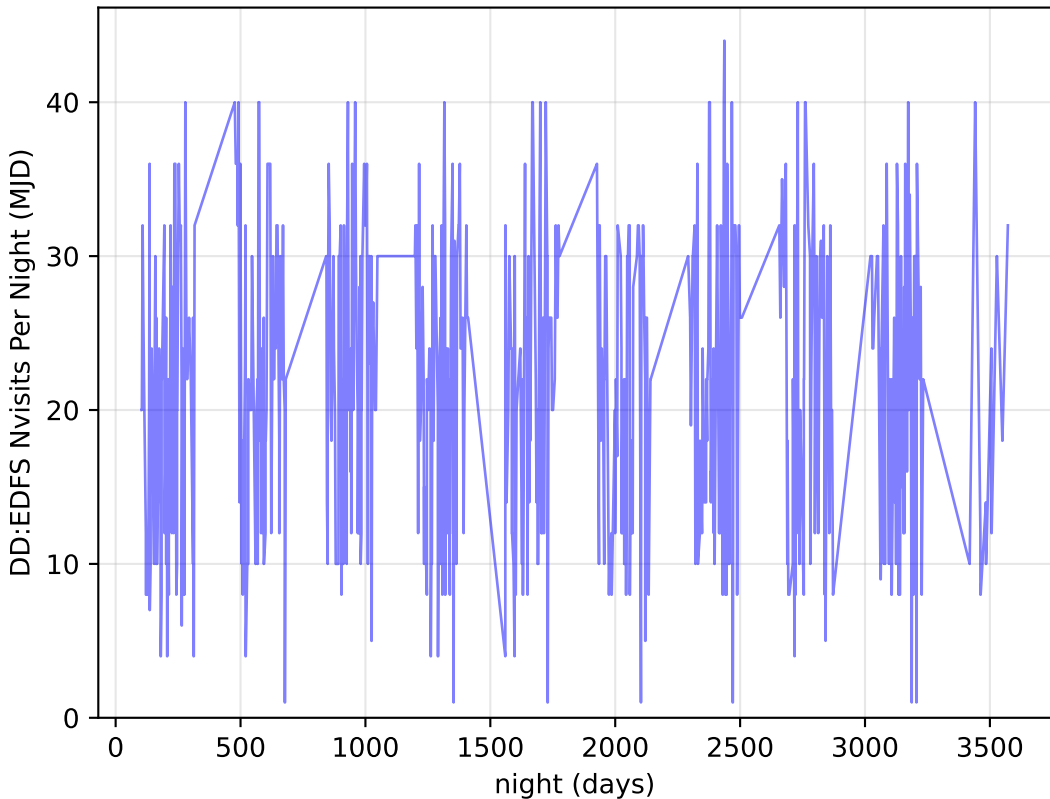
ddf_loaded_half_fl1_v3.4_10yrs all bands: DD:EDFS Nvisits Per Night
