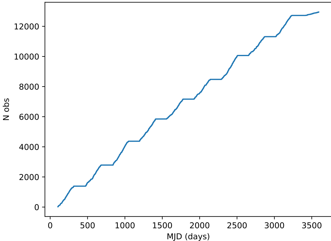
ddf_loaded_half_fl1_v3.4_10yrs all bands: DD:EDFS Cumulative NVisits
