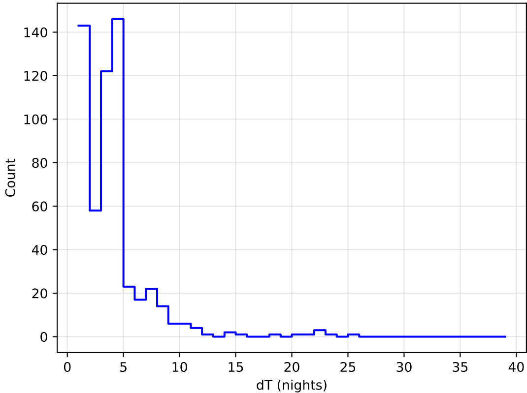
ddf_loaded_half_fl1_v3.4_10yrs all bands: DD:ECDFS Delta Nights Histogram
