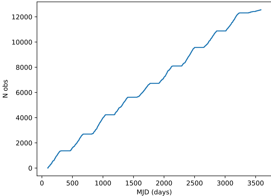
ddf_loaded_half_fl1_v3.4_10yrs all bands: DD:ECDFS Cumulative NVisits
