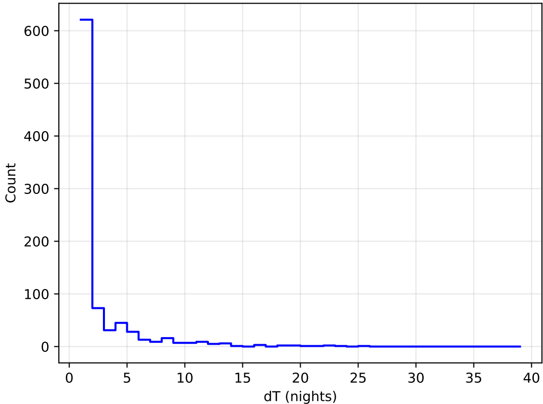
ddf_loaded_half_fl1_v3.4_10yrs all bands: DD:COSMOS Delta Nights Histogram
