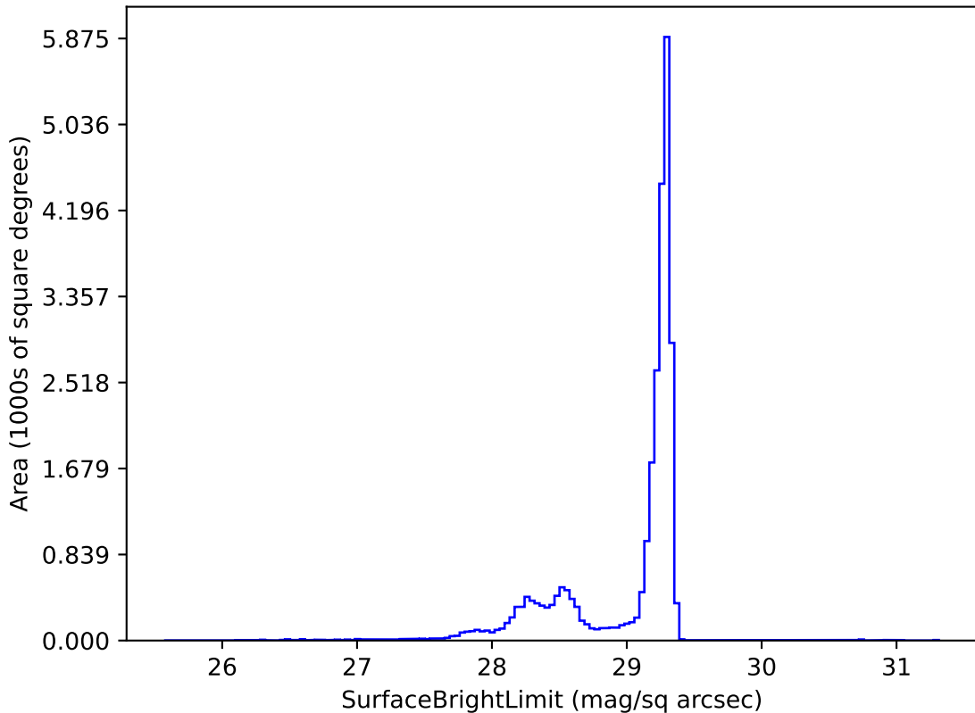
ddf_loaded_half_fl1_v3.3_10yrs z: SurfaceBrightLimit
