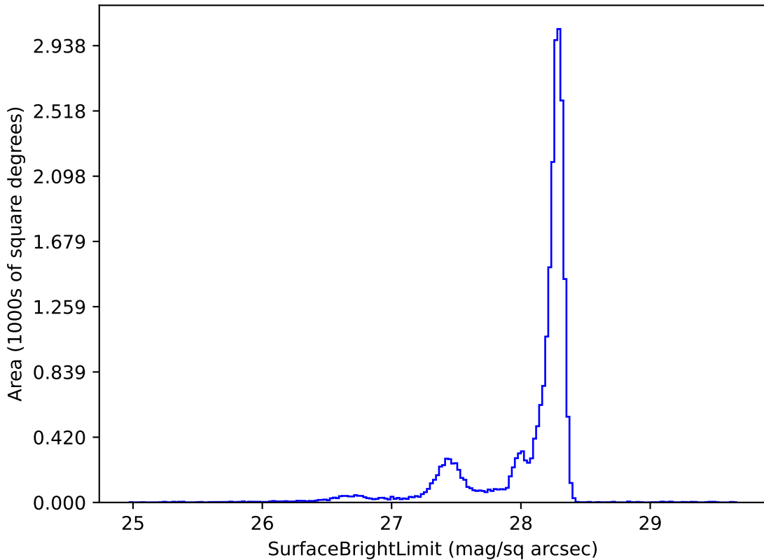
ddf_loaded_half_fl1_v3.3_10yrs y: SurfaceBrightLimit
