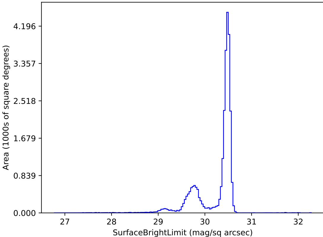
ddf_loaded_half_fl1_v3.3_10yrs r: SurfaceBrightLimit
