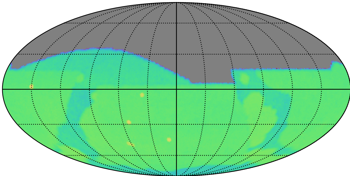
ddf_loaded_half_fl1_v3.3_10yrs g: SurfaceBrightLimit
