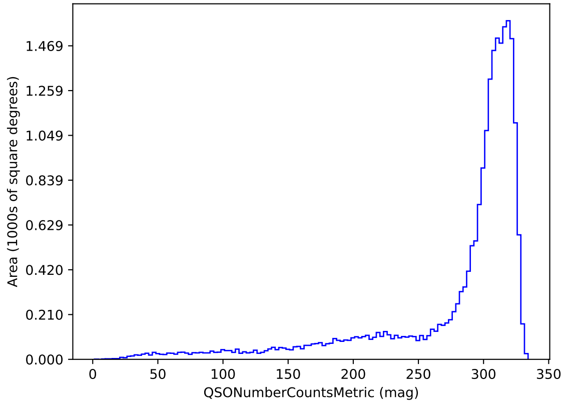
ddf_loaded_half_fl1_v3.3_10yrs u band and non-DD: QSONumberCountsMetric
