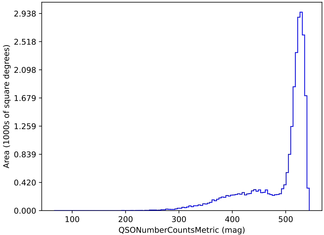
ddf_loaded_half_fl1_v3.3_10yrs r band and non-DD: QSONumberCountsMetric
