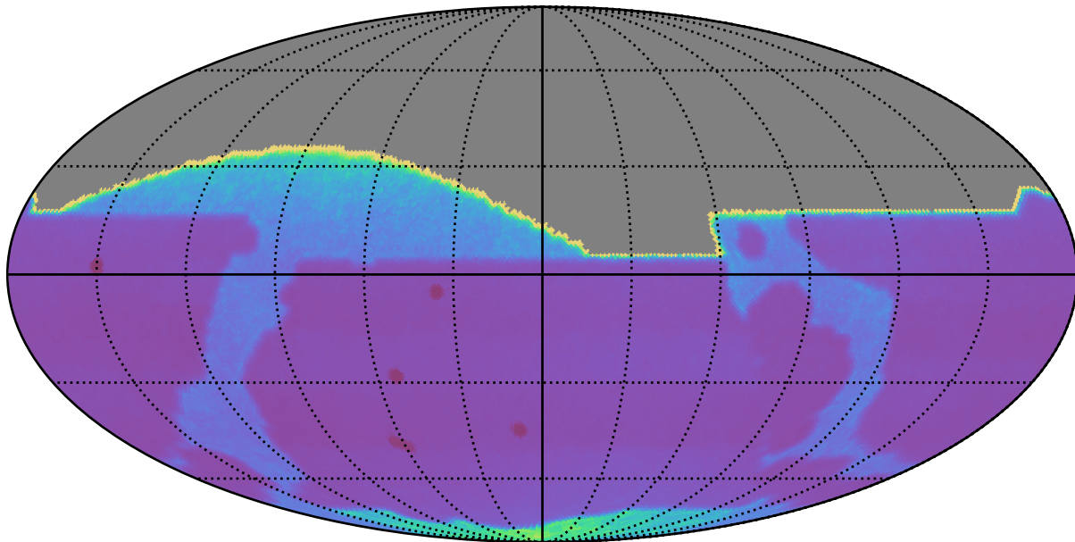
ddf_loaded_half_fl1_v3.3_10yrs : Proper Motion Uncert @ 20.5
