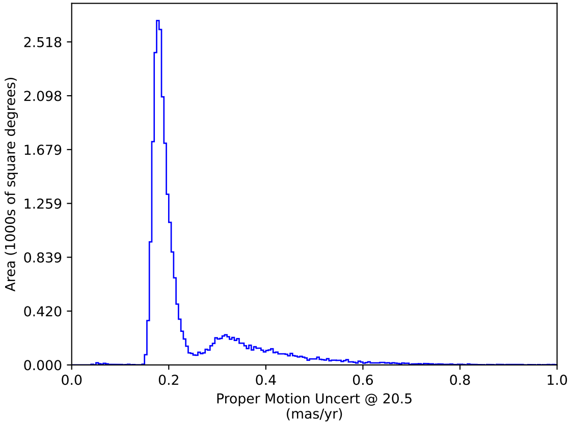
ddf_loaded_half_fl1_v3.3_10yrs : Proper Motion Uncert @ 20.5
