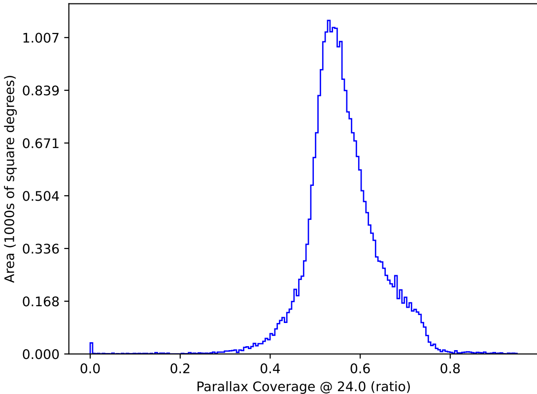
ddf_loaded_half_fl1_v3.3_10yrs : Parallax Coverage @ 24.0
