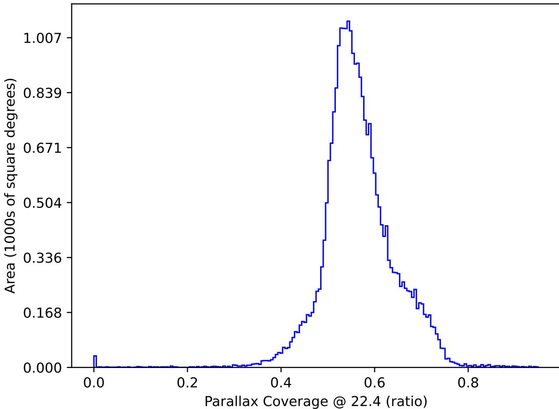
ddf_loaded_half_fl1_v3.3_10yrs : Parallax Coverage @ 22.4
