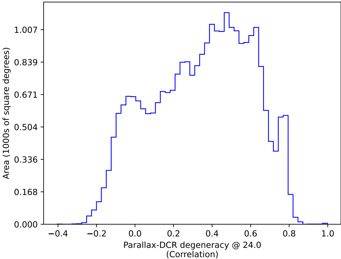
ddf_loaded_half_fl1_v3.3_10yrs : Parallax-DCR degeneracy @ 24.0
