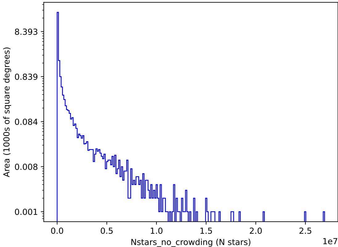
ddf_loaded_half_fl1_v3.3_10yrs z: Nstars_no_crowding
