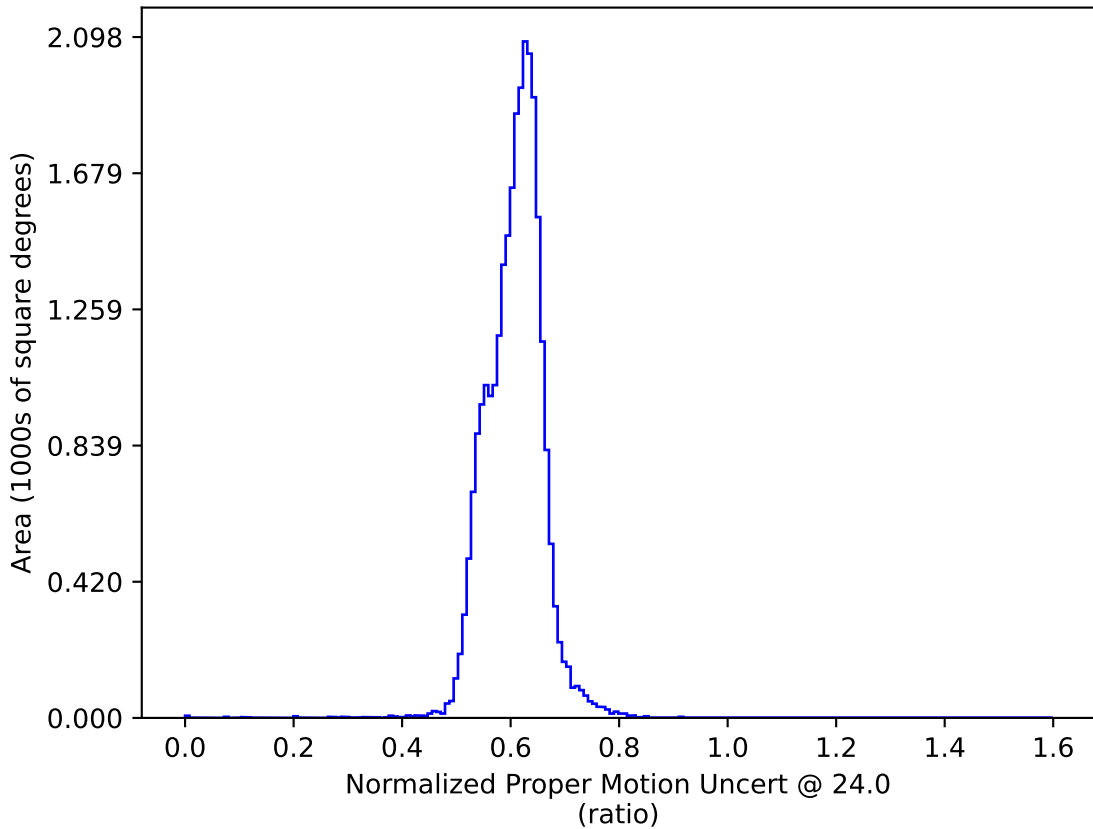
ddf_loaded_half_fl1_v3.3_10yrs : Normalized Proper Motion Uncert @ 24.0
