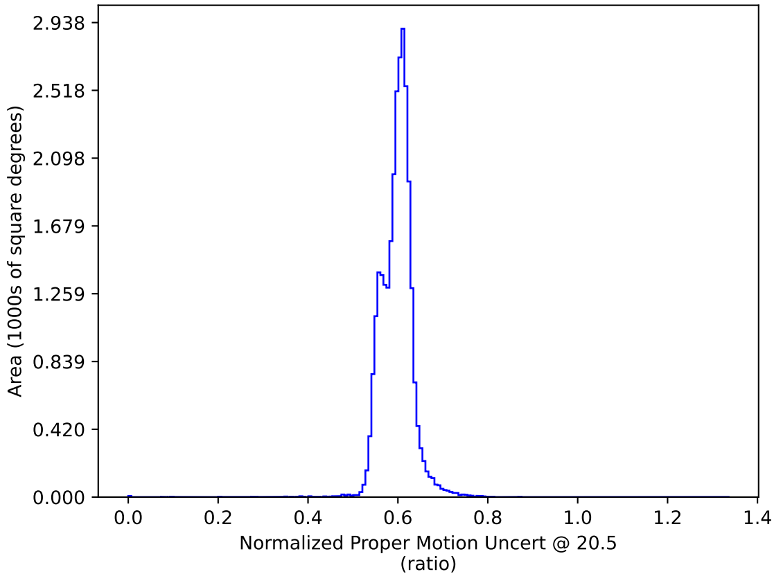
ddf_loaded_half_fl1_v3.3_10yrs : Normalized Proper Motion Uncert @ 20.5
