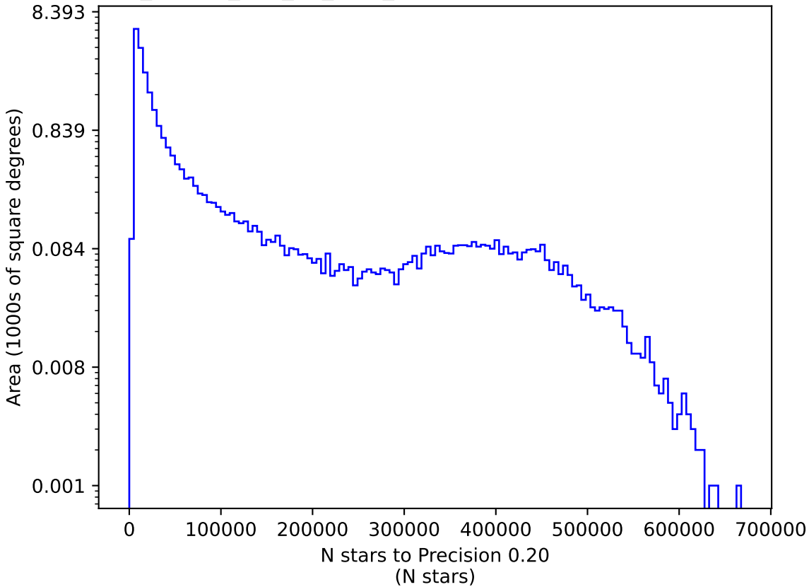
ddf_loaded_half_fl1_v3.3_10yrs z: N stars to Precision 0.20
