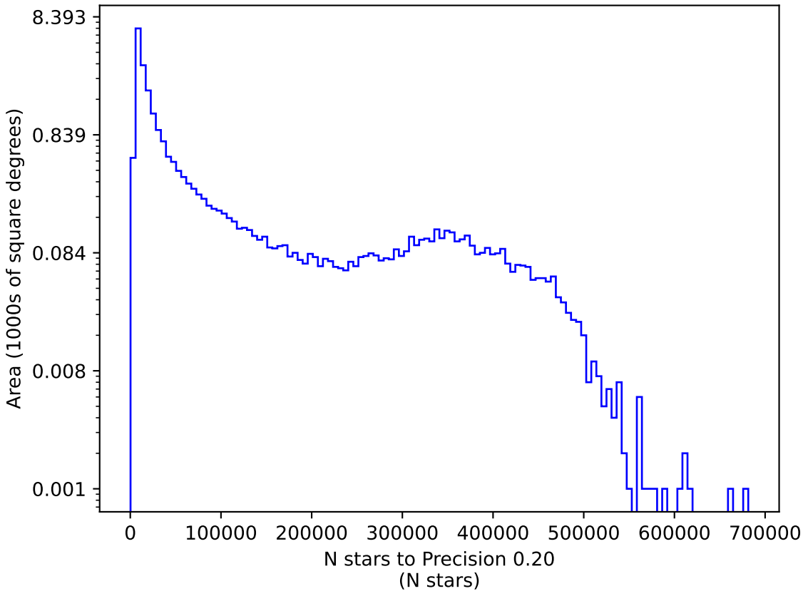
ddf_loaded_half_fl1_v3.3_10yrs y: N stars to Precision 0.20
