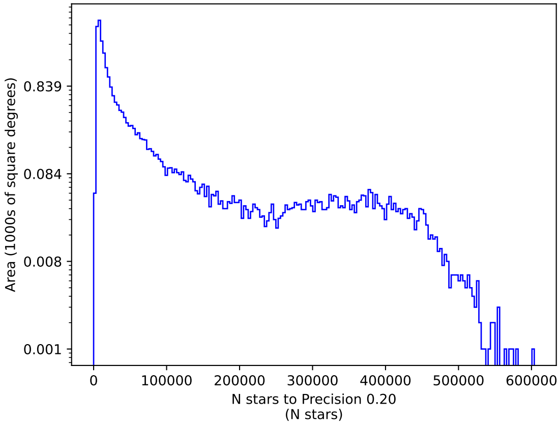
ddf_loaded_half_fl1_v3.3_10yrs g: N stars to Precision 0.20
