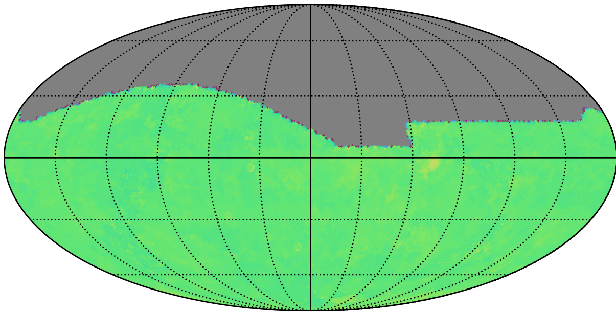
ddf_loaded_half_fl1_v3.3_10yrs g: Kuiper rotTelPos
