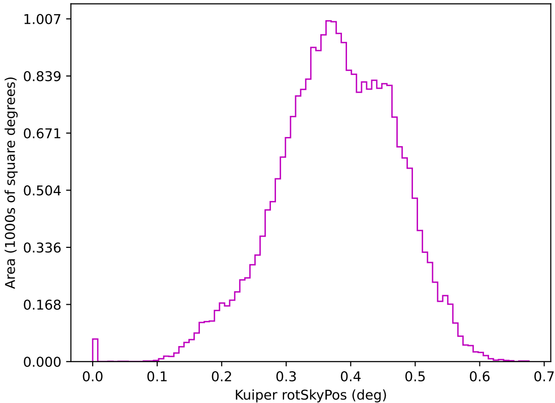
ddf_loaded_half_fl1_v3.3_10yrs z: Kuiper rotSkyPos
