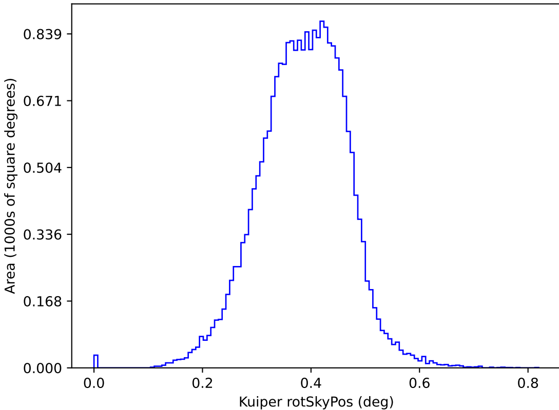
ddf_loaded_half_fl1_v3.3_10yrs y: Kuiper rotSkyPos
