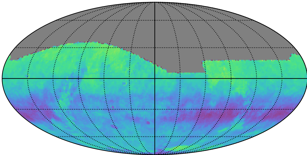
ddf_loaded_half_fl1_v3.3_10yrs r: Kuiper rotSkyPos
