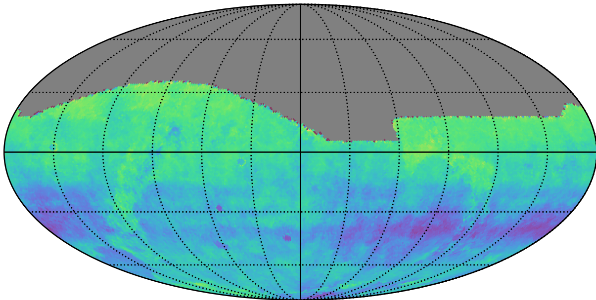
ddf_loaded_half_fl1_v3.3_10yrs i: Kuiper rotSkyPos
