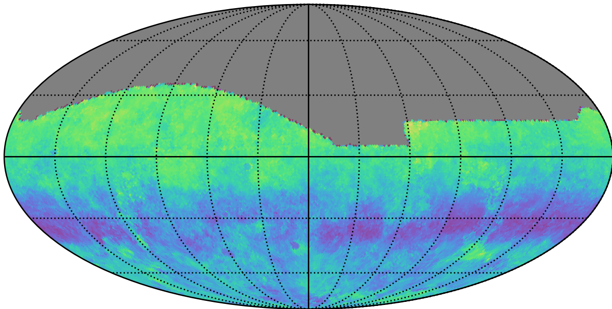
ddf_loaded_half_fl1_v3.3_10yrs g: Kuiper rotSkyPos
